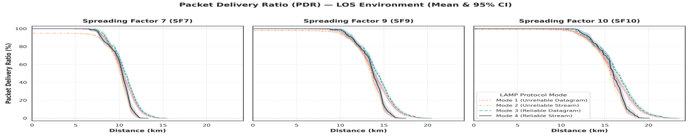
Fig. 5. Packet Delivery Ratio ( PDR_{app} %) as a function of distance across Spreading Factors (SF7, SF9, SF10) in Line-of-Sight (LoS) propagation. Solid lines denote mean delivery rates across 50 Monte Carlo trials; shaded ribbons represent 95% confidence intervals.
