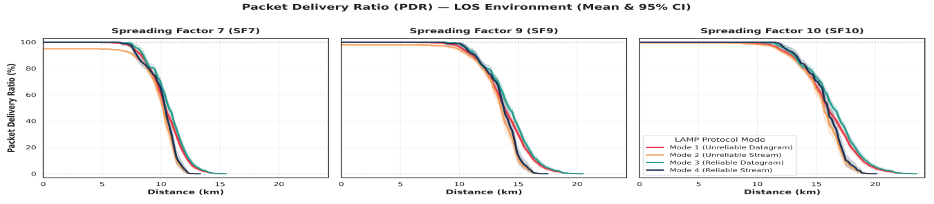
Fig. 5. Packet Delivery Ratio (PDR %) as a function of distance across Spreading Factors (SF7, SF9, SF10) in Line-of-Sight (LoS) propagation. Solid lines denote mean delivery rates across 50 Monte Carlo trials; shaded ribbons represent 95% confidence intervals.
