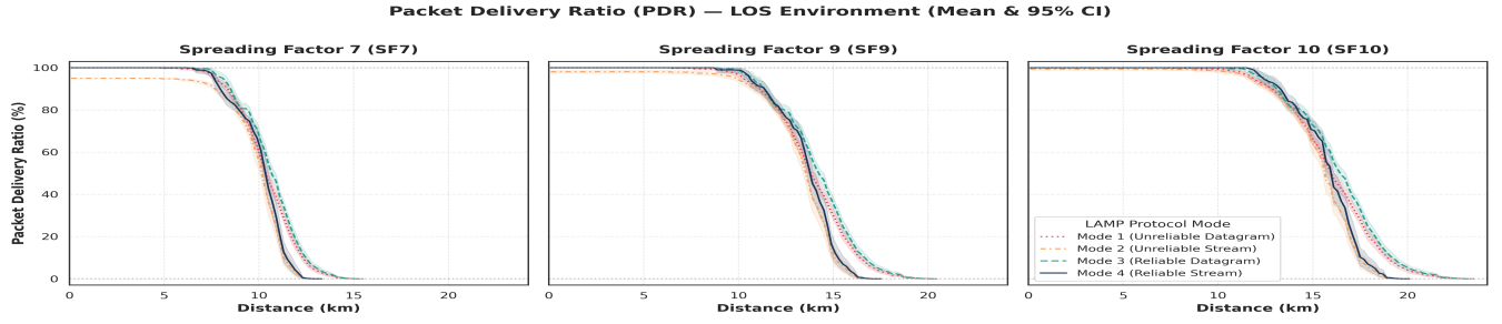
Fig. 5. Packet Delivery Ratio ( PDR_{app} %) as a function of distance across Spreading Factors (SF7, SF9, SF10) in Line-of-Sight (LoS) propagation. Solid lines denote mean delivery rates across 50 Monte Carlo trials; shaded ribbons represent 95% confidence intervals.
