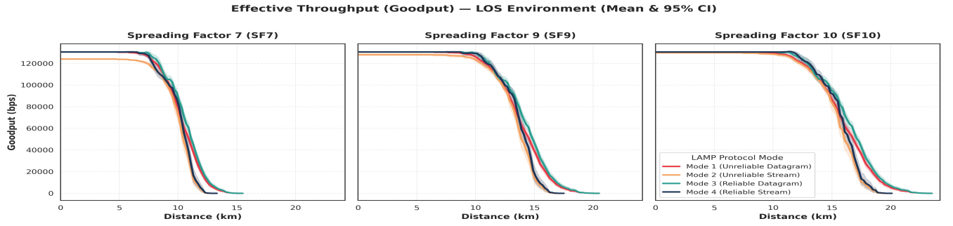
Fig. 6. Effective application-layer throughput (Goodput in bps) across Spreading Factors and LAMP operational modes in LoS. Shaded ribbons denote 95% confidence intervals across 50 Monte Carlo trials.
