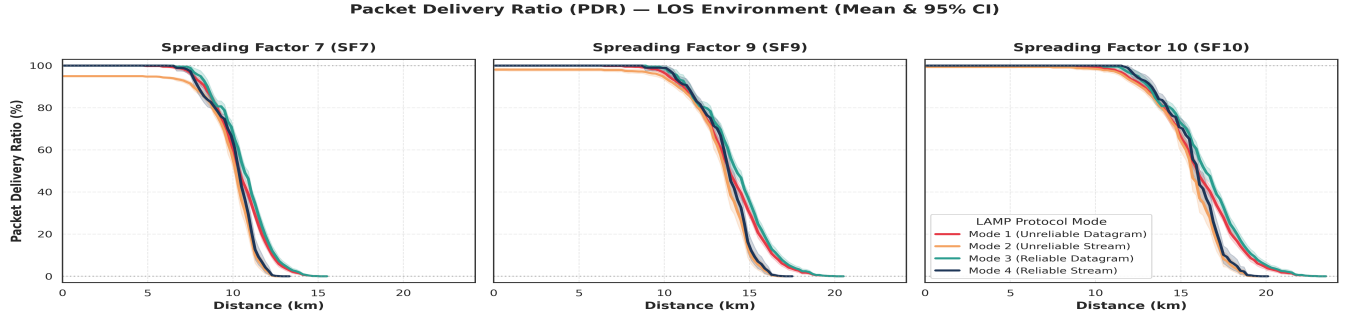
Fig. 5. Packet Delivery Ratio (PDR %) as a function of distance across Spreading Factors (SF7, SF9, SF10) in Line-of-Sight (LoS) propagation. Solid lines denote mean delivery rates across 50 Monte Carlo trials; shaded ribbons represent 95% confidence intervals.
