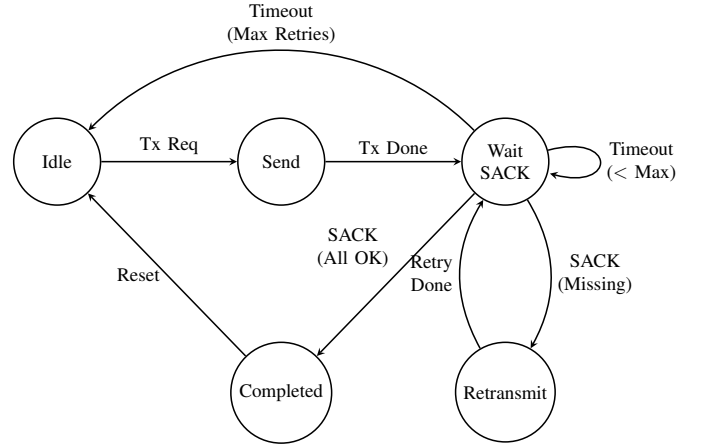
Fig. 2. State machine of the reliable transmission process at the transmitter.
