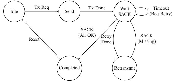
Fig. 2. State machine of the reliable transmission process at the transmitter.
