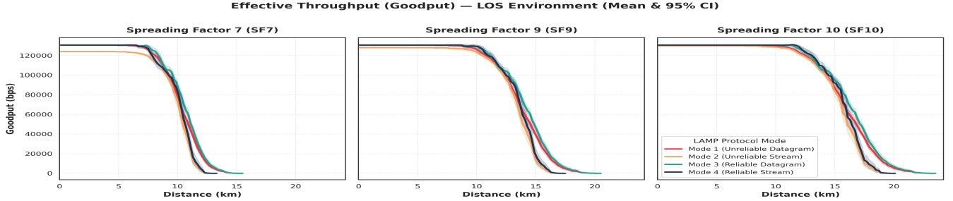
Fig. 6. Effective application-layer throughput (Goodput in bps) across Spreading Factors and LAMP operational modes in LoS. Shaded ribbons denote 95% confidence intervals across 50 Monte Carlo trials.
