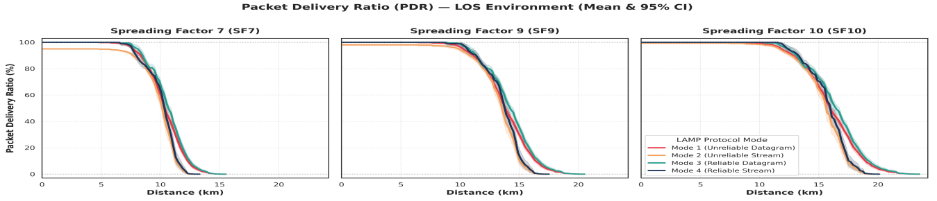
Fig. 5. Packet Delivery Ratio (PDR %) as a function of distance across Spreading Factors (SF7, SF9, SF10) in Line-of-Sight (LoS) propagation. Solid lines denote mean delivery rates across 50 Monte Carlo trials; shaded ribbons represent 95% confidence intervals.
