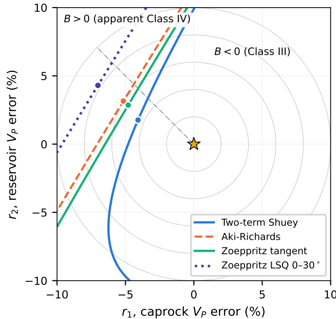
Figure 5. Class III/IV boundary ( B = 0 ) in the (r_1, r_2) error plane for two-term Shuey, Aki-Richards, the exact Zoeppritz tangent, and the 0^\circ – 30^\circ least-squares Zoeppritz gradient. Dots mark each boundary’s closest approach to the baseline (star); the dash-dotted line is the \phi = 135^\circ spoke; grey circles are |r| = 2\% – 10\% .
