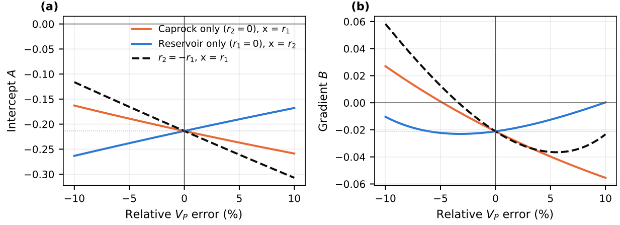
Figure 1. (a) Intercept A and (b) two-term Shuey gradient B versus relative V_P error for caprock-only ( r_2 = 0 ), reservoir-only ( r_1 = 0 ), and r_2 = -r_1 perturbations. Shale over \text{CO}_2 sand; \sigma is recomputed at each perturbed velocity. Dotted lines mark the baseline values.
