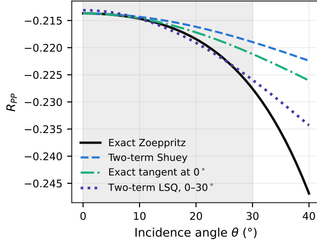
Figure 4. Exact Zoeppritz R_{PP}(\theta) at the baseline (shale over CO 2 sand) compared with the two-term Shuey curve, the exact normal-incidence tangent, and the two-term least-squares fit over 0°–30° (shaded).
