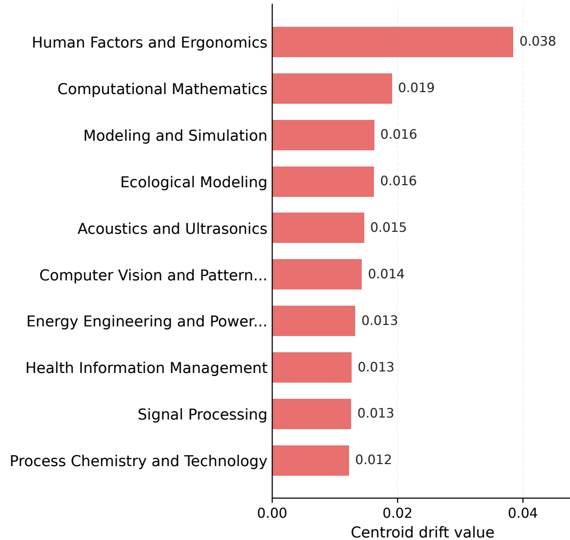
Highest early--late centroid drift
