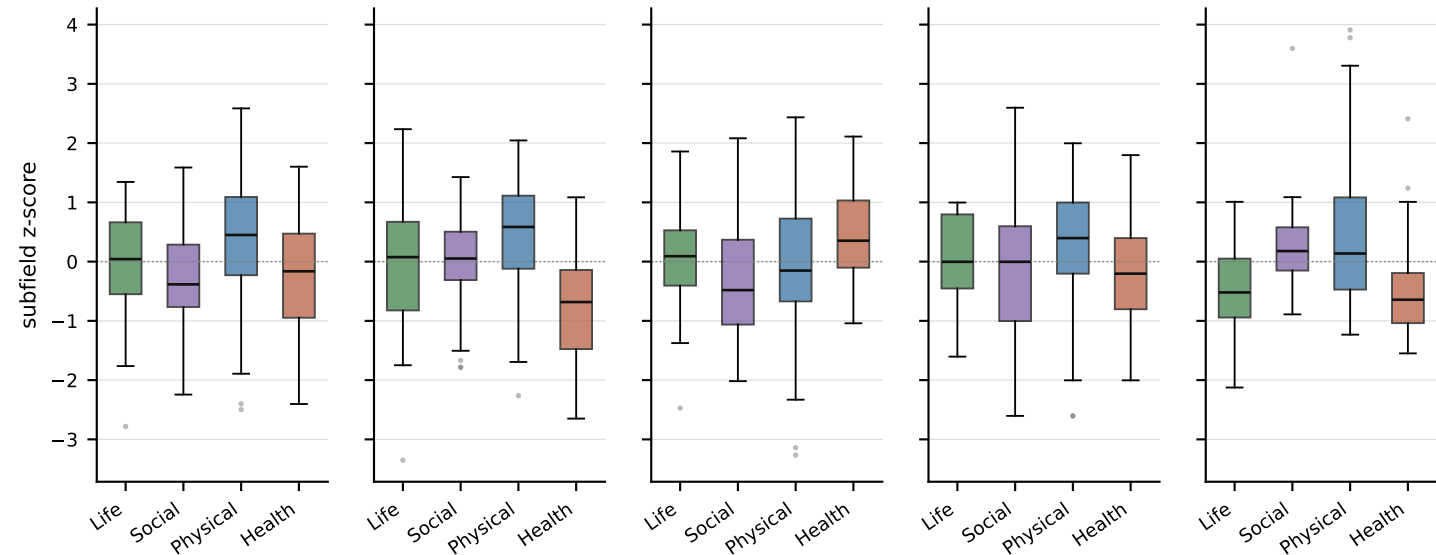
Centroid median
