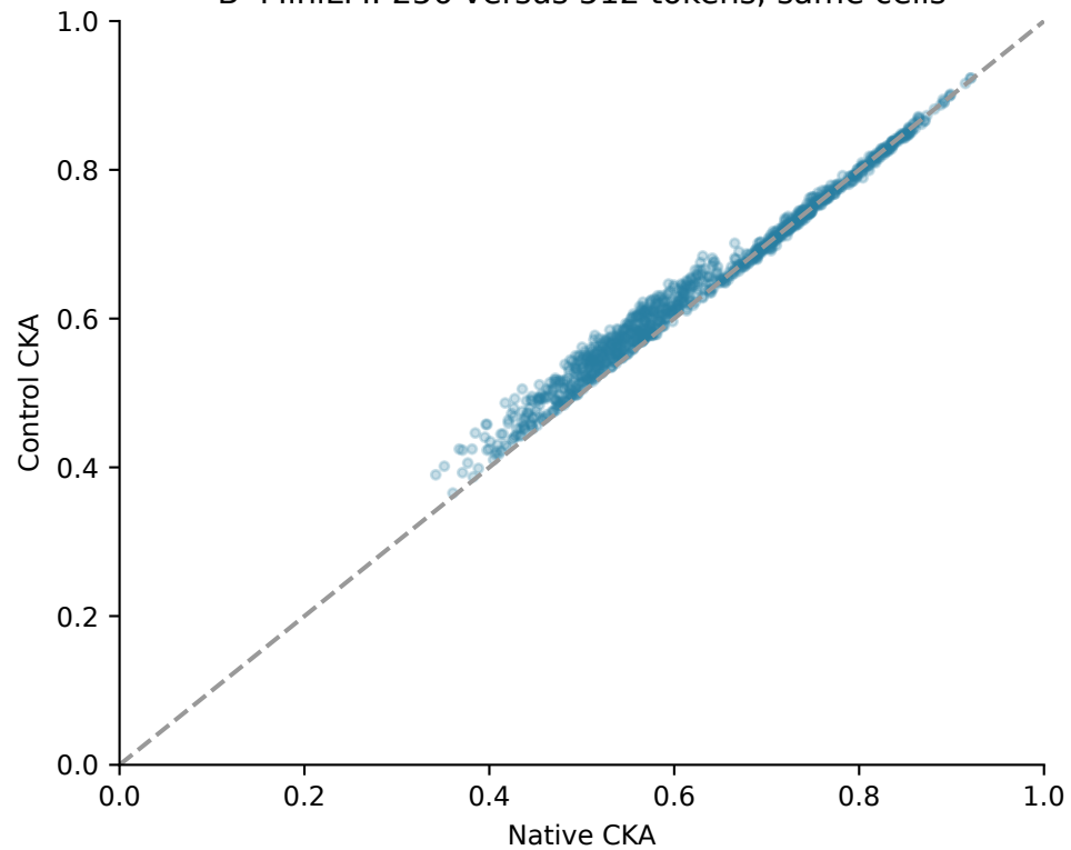
B MiniLM: 256 versus 512 tokens; same cells
