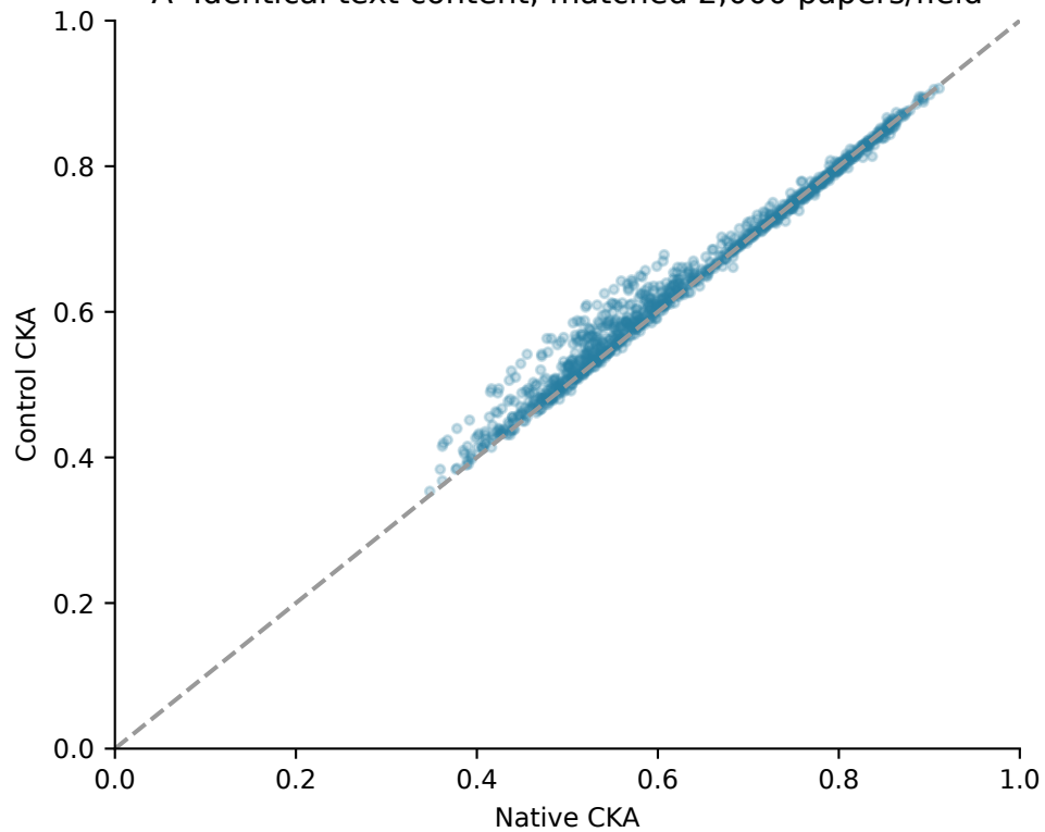
A Identical text content; matched 2,000 papers/field
