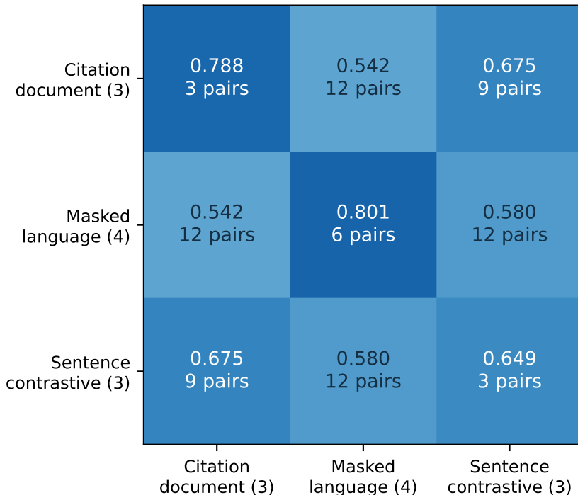
A Shape agreement
