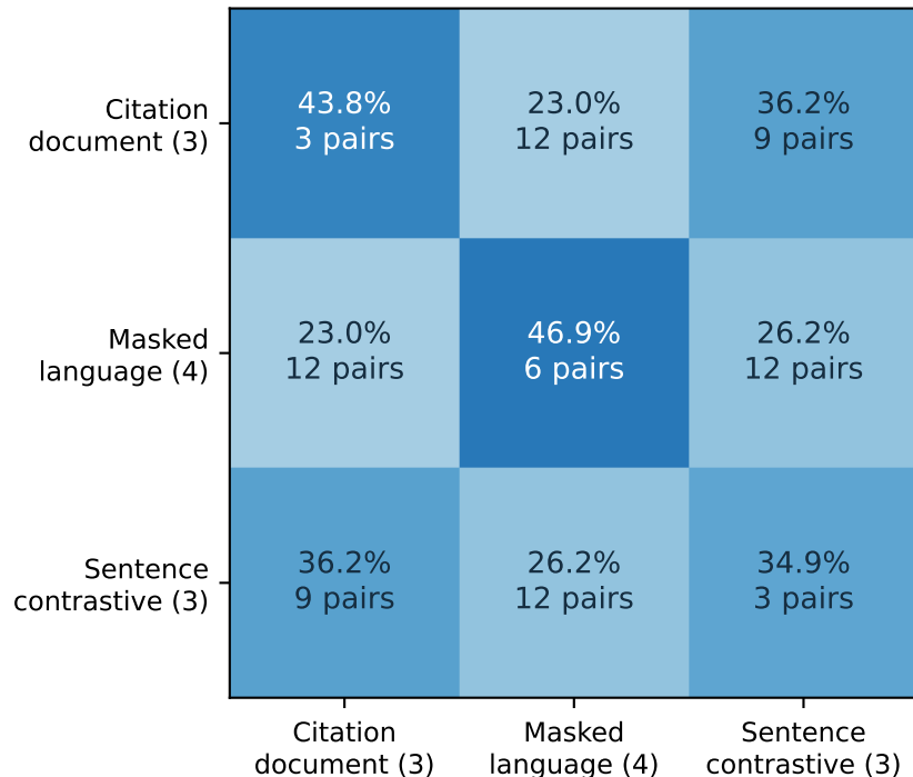
B Shared top-25 neighbors (%)
