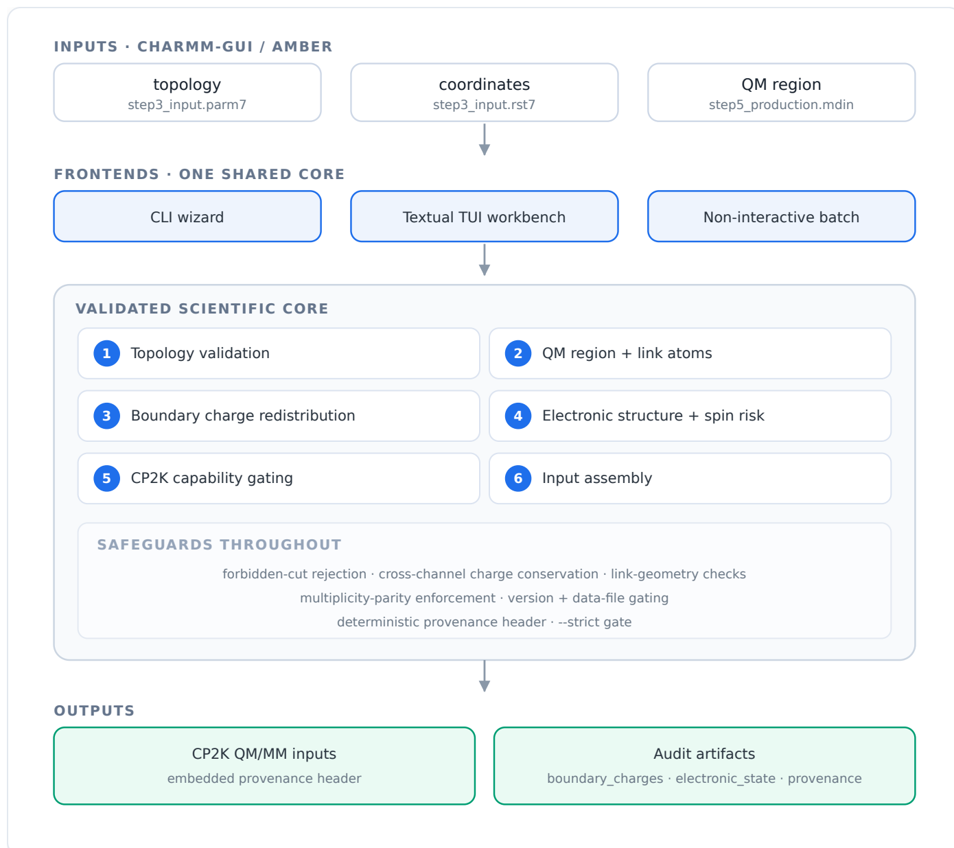
Figure 1. Architecture and data flow. Three frontends share one validated scientific core that ingests CHARMM-GUI/AMBER inputs, applies six sequential stages under cross-cutting safeguards, and emits runnable CP2K QM/MM input plus machine- and human-readable audit artifacts.
