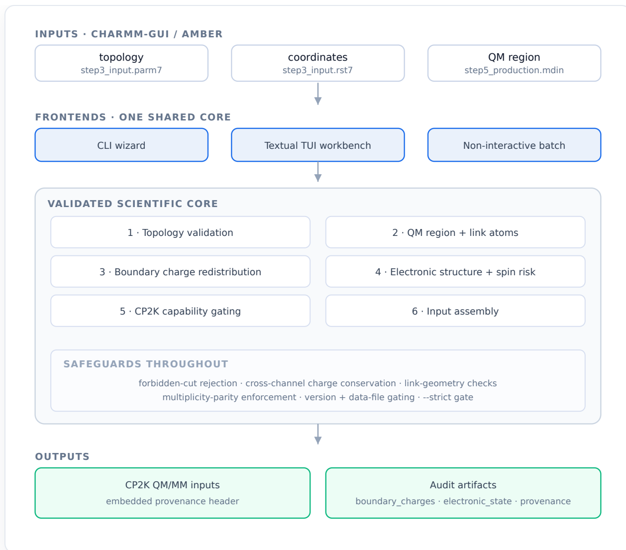
Figure 1. Architecture and data flow. Three frontends share one validated scientific core that ingests CHARMM-GUI/AMBER inputs, applies six sequential stages under cross-cutting safeguards, and emits runnable CP2K QM/MM input plus machine- and human-readable audit artifacts.
