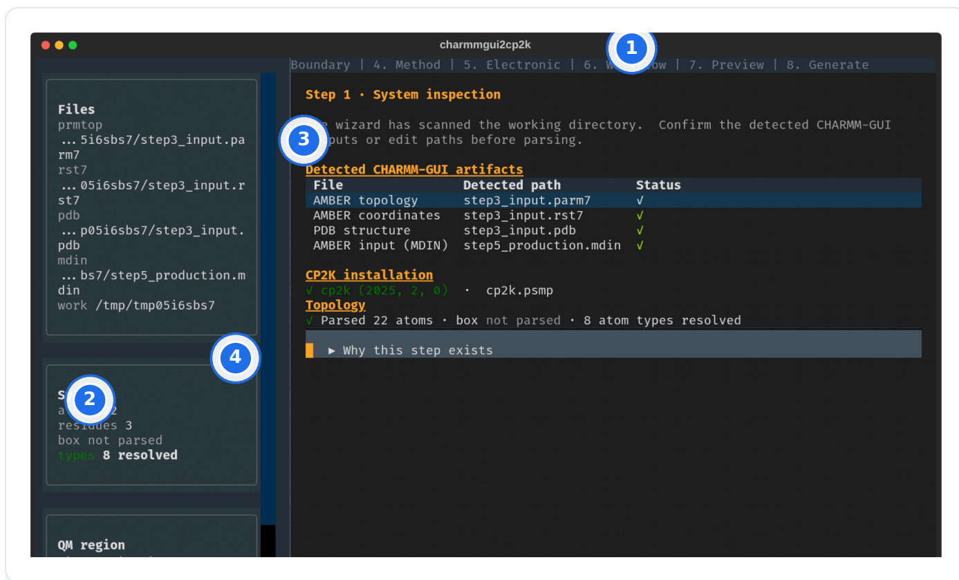
Figure 2. The Textual TUI workbench (rendered live, headlessly) on the System phase. Callouts: (1) the phase rail showing current and remaining steps; (2) the sticky system summary; (3) auto-detected inputs, each with its provenance; (4) progressive disclosure of expert detail. Keyboard-first navigation makes the next safe action obvious without a manual.
