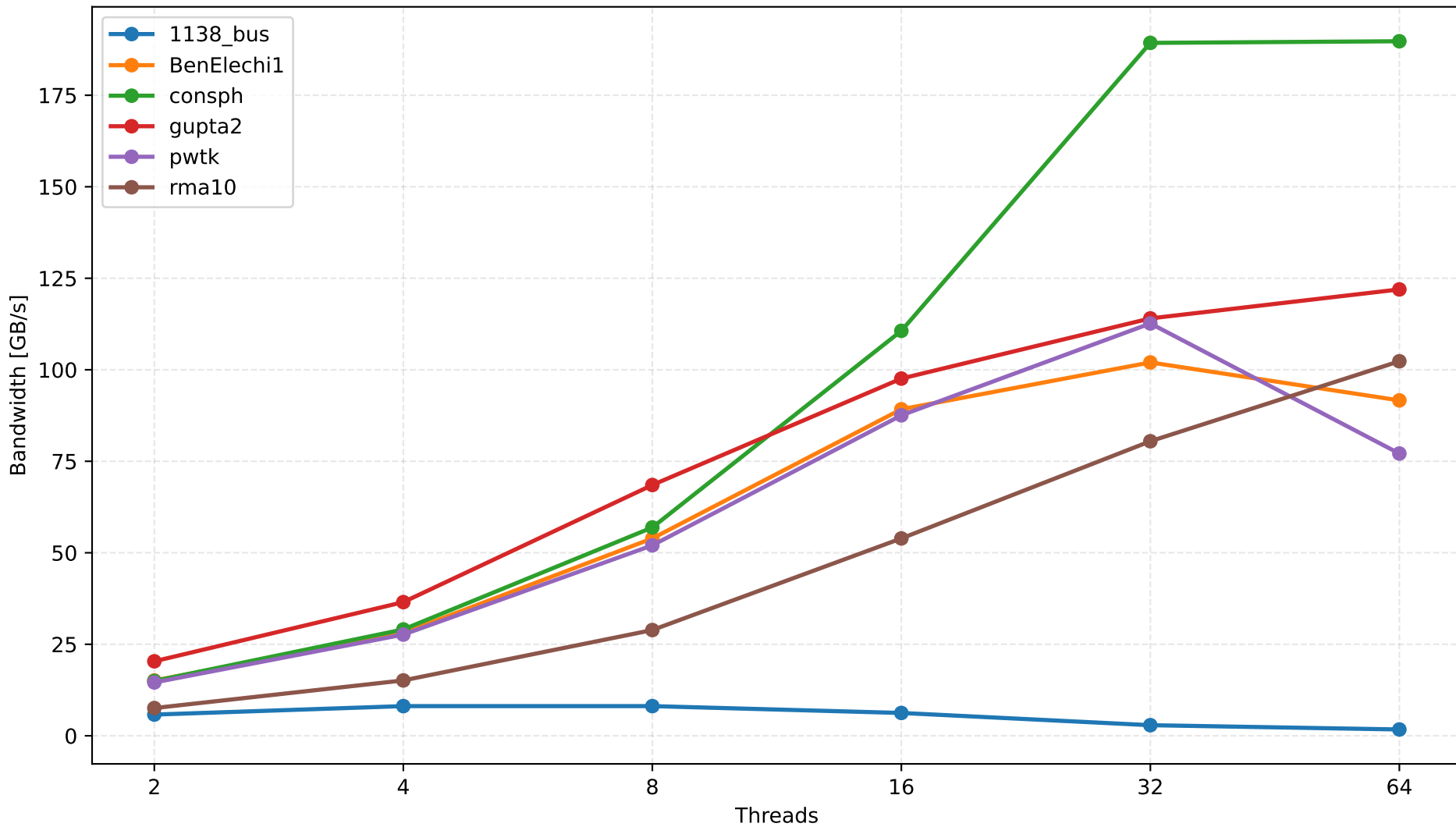
Achieved Memory Bandwidth Across All Matrices
