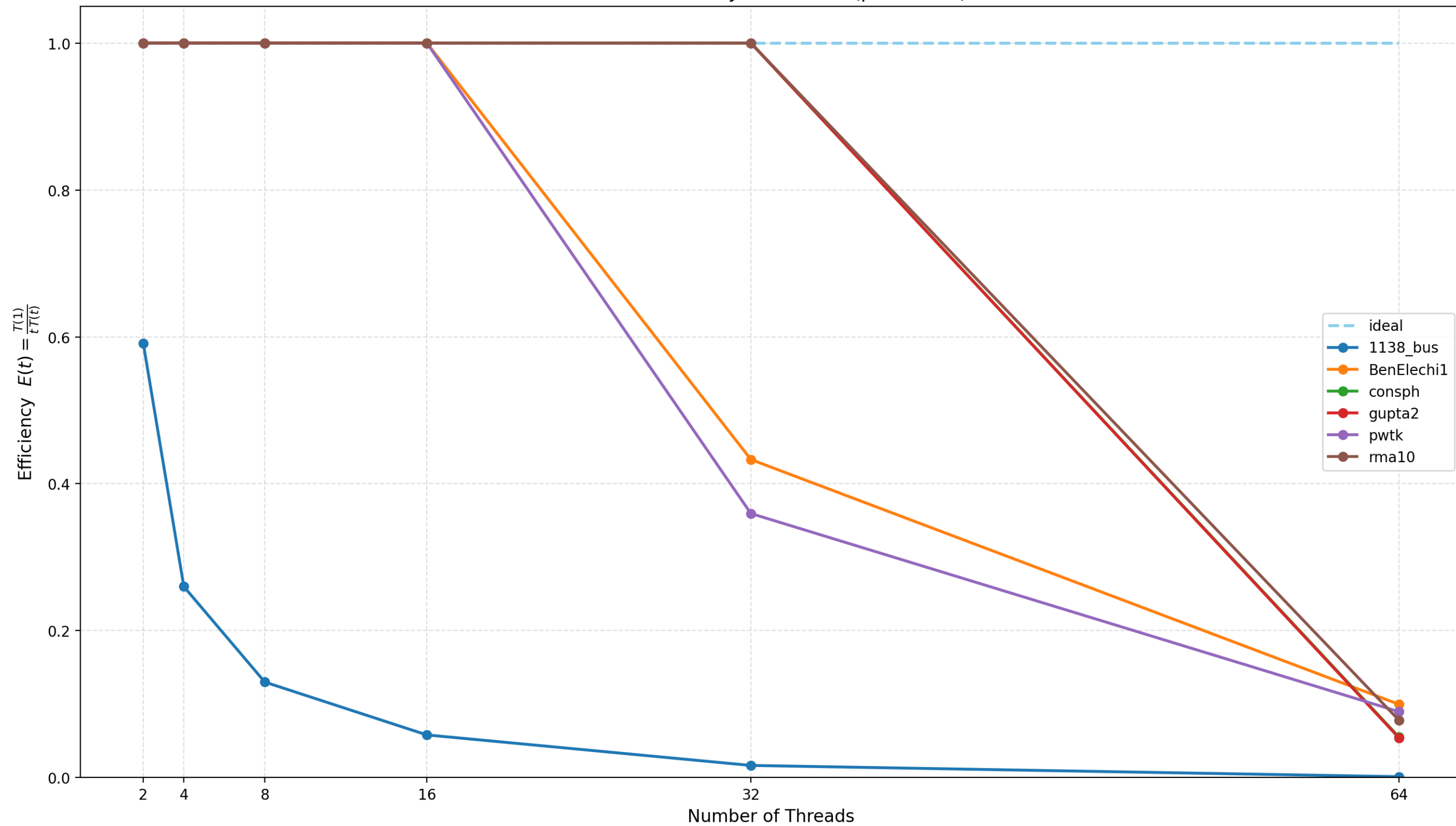
Parallel Efficiency vs Threads (p90-based)
