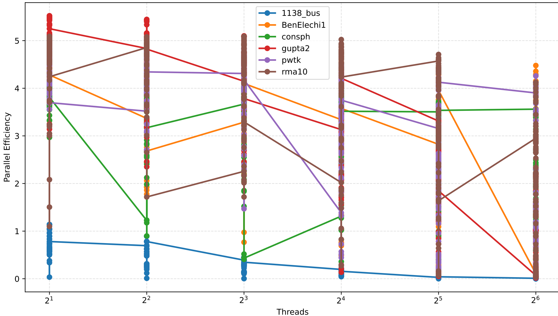
Parallel Efficiency vs Threads for All Matrices
