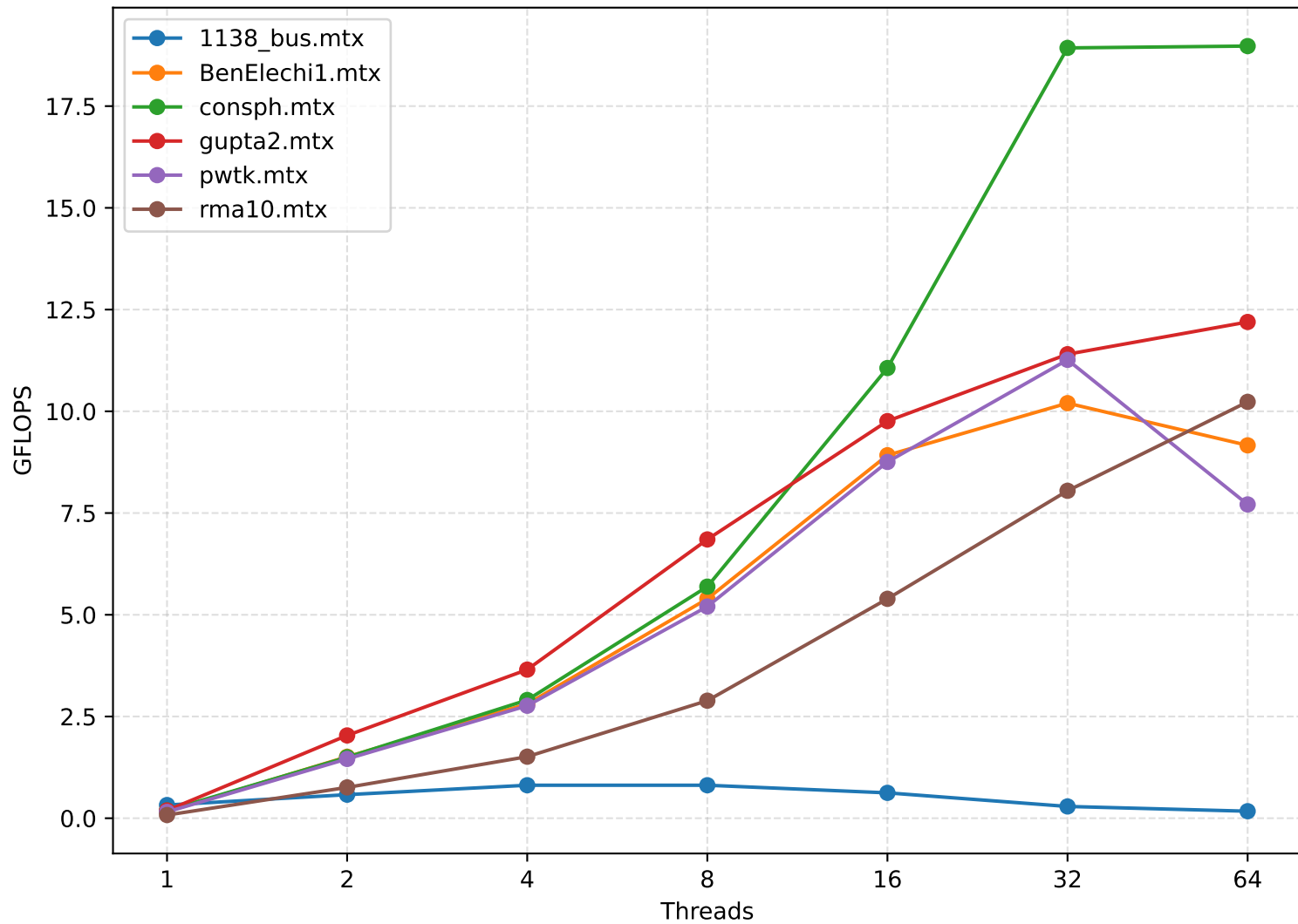
GFLOPS vs Threads per Matrix (CSR SpMV)
