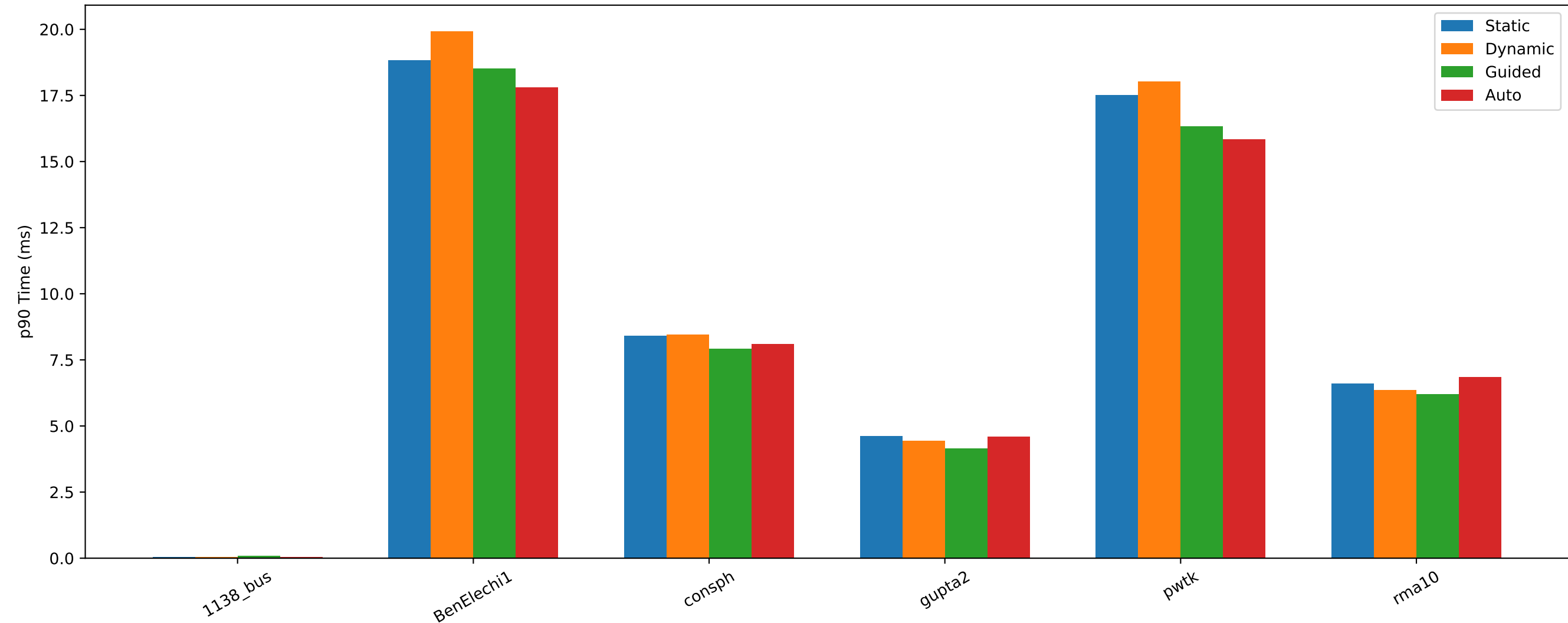
Scheduling Comparison Across All Matrices (p90 Execution Time)
