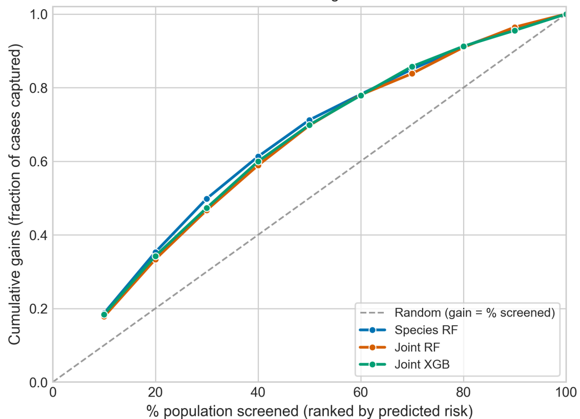
Cumulative gains
