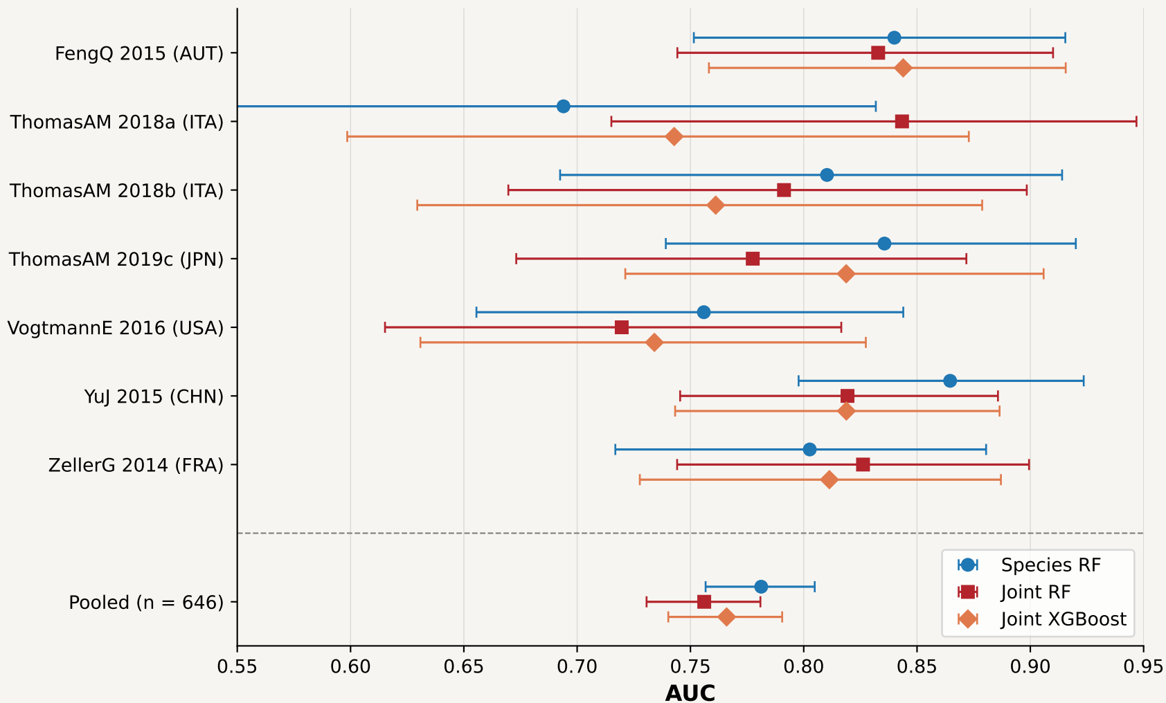
Figure 1. Per-cohort and pooled AUC with 95% bootstrap CI under LODO cross-validation
