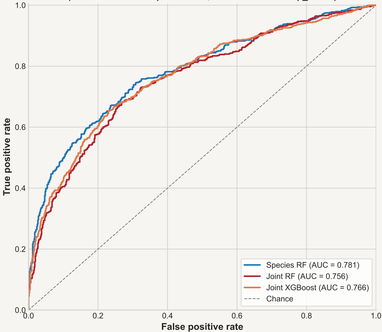
Figure 2. Pooled LODO ROC curves (10-cohort hold-out predictions; AUC from bootstrap_ci.csv)
