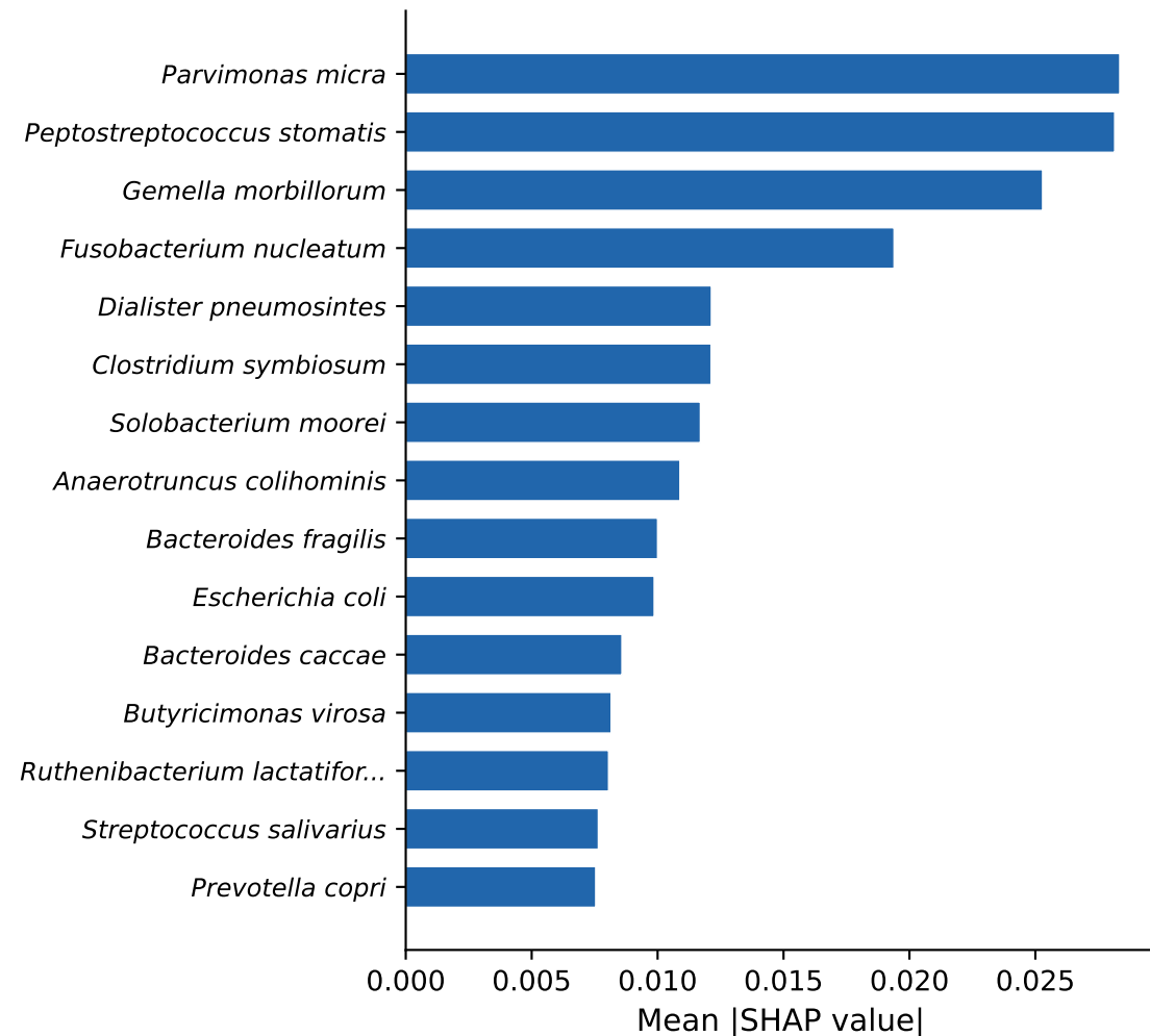
Random Forest
