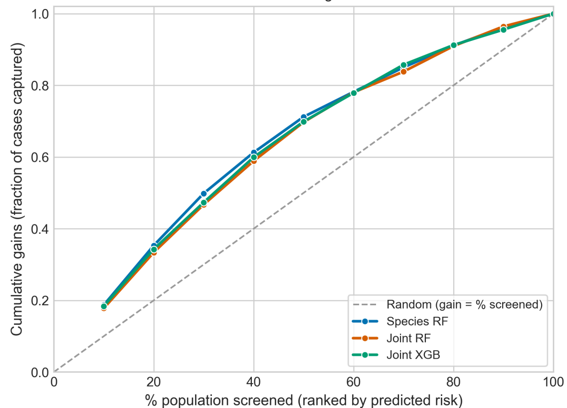
Cumulative gains
