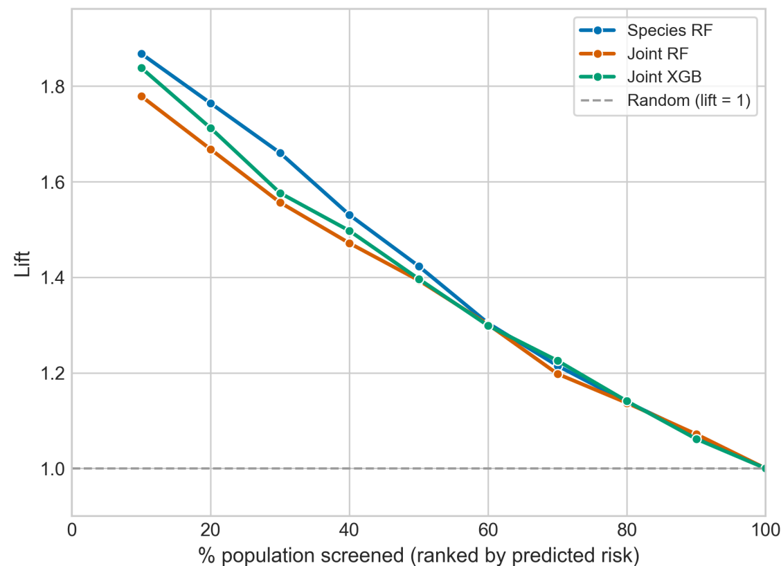
Lift curve
