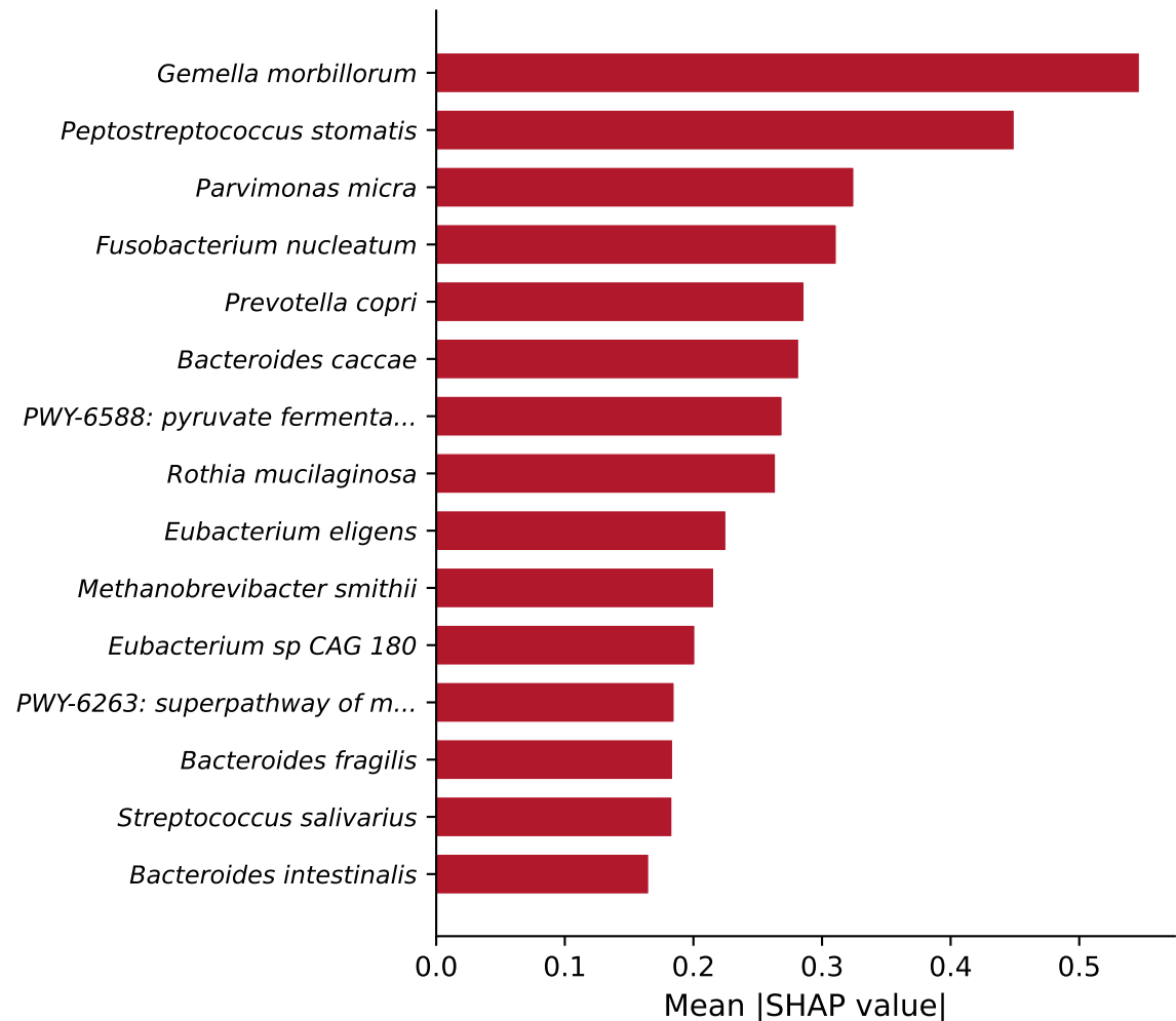
XGBoost
