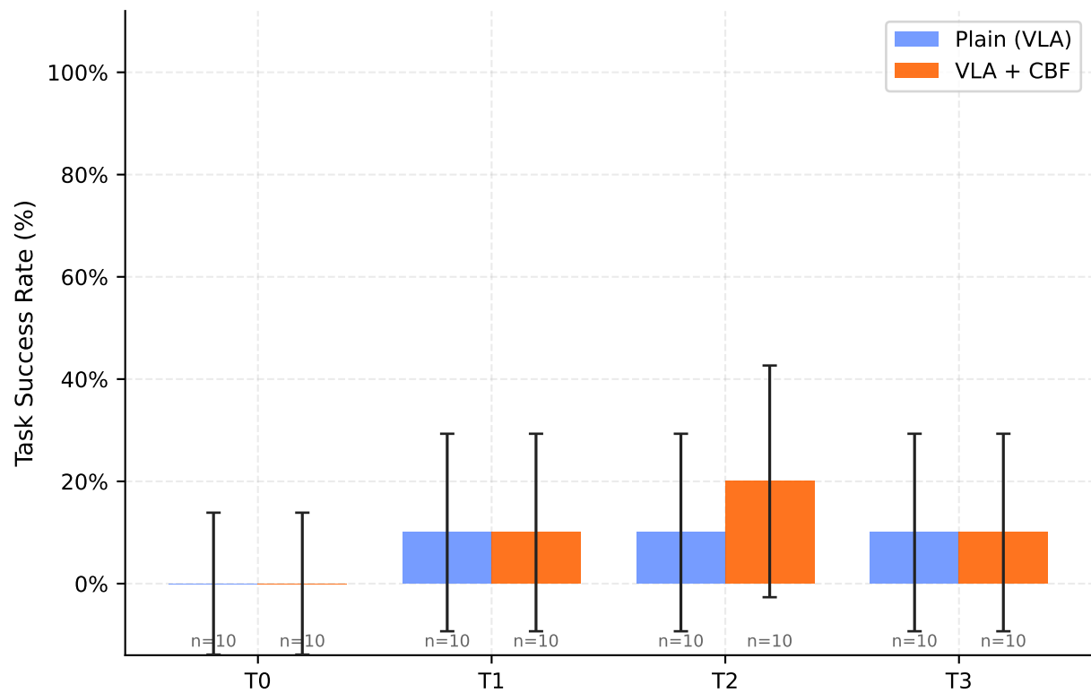
SafeLIBERO-Spatial LI · Task Success Rate
