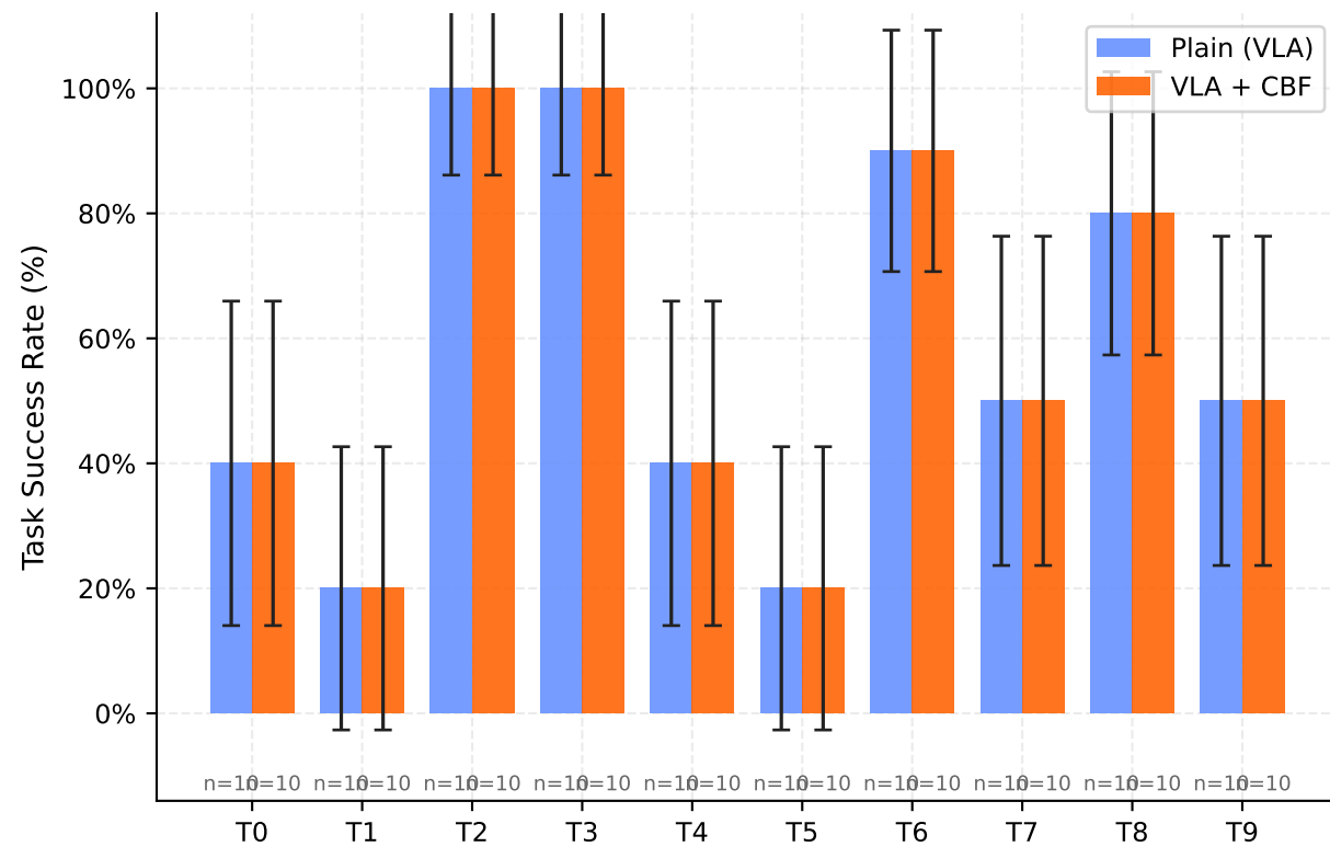
LIBERO-Spatial · Task Success Rate
