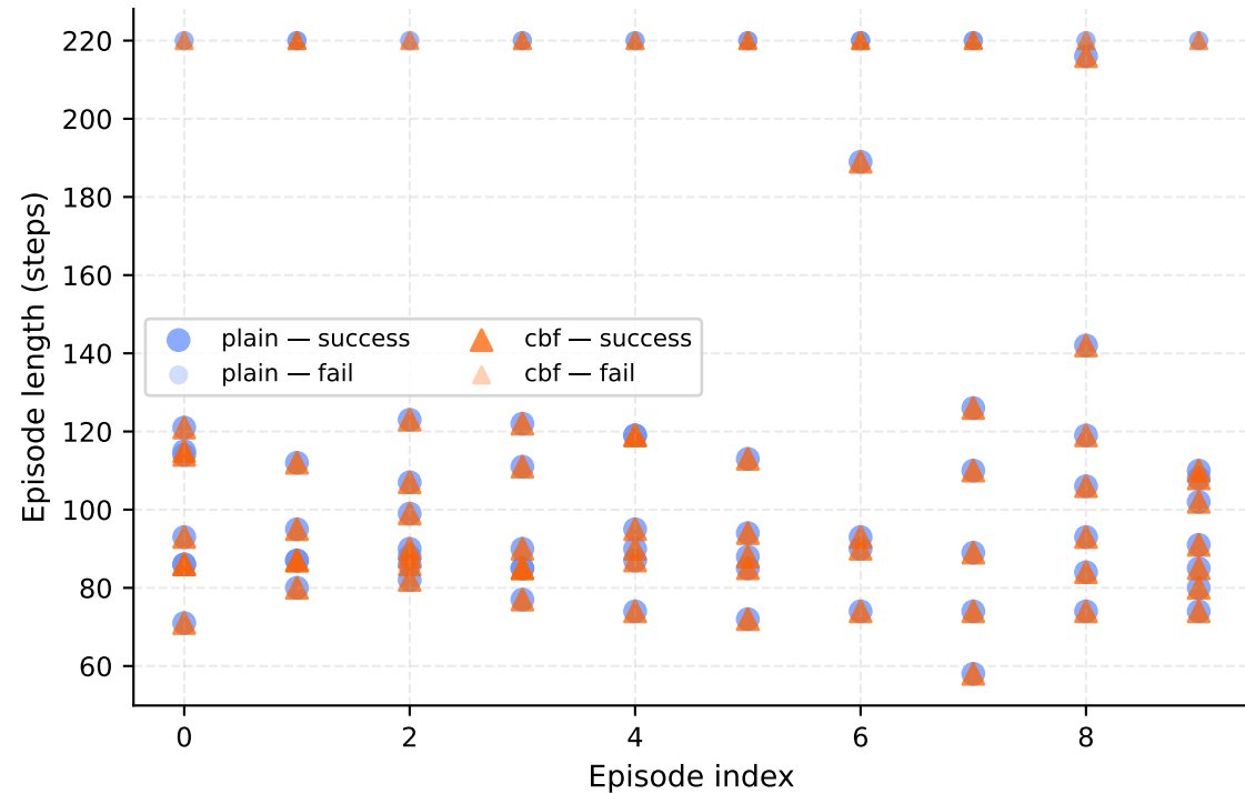
LIBERO-Spatial
