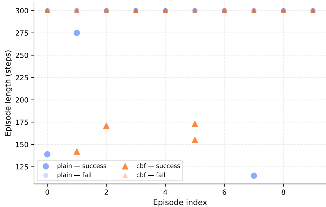
SafeLIBERO-Spatial LI
