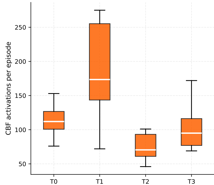
CBF Filter Activations (VLA + CBF mode)
