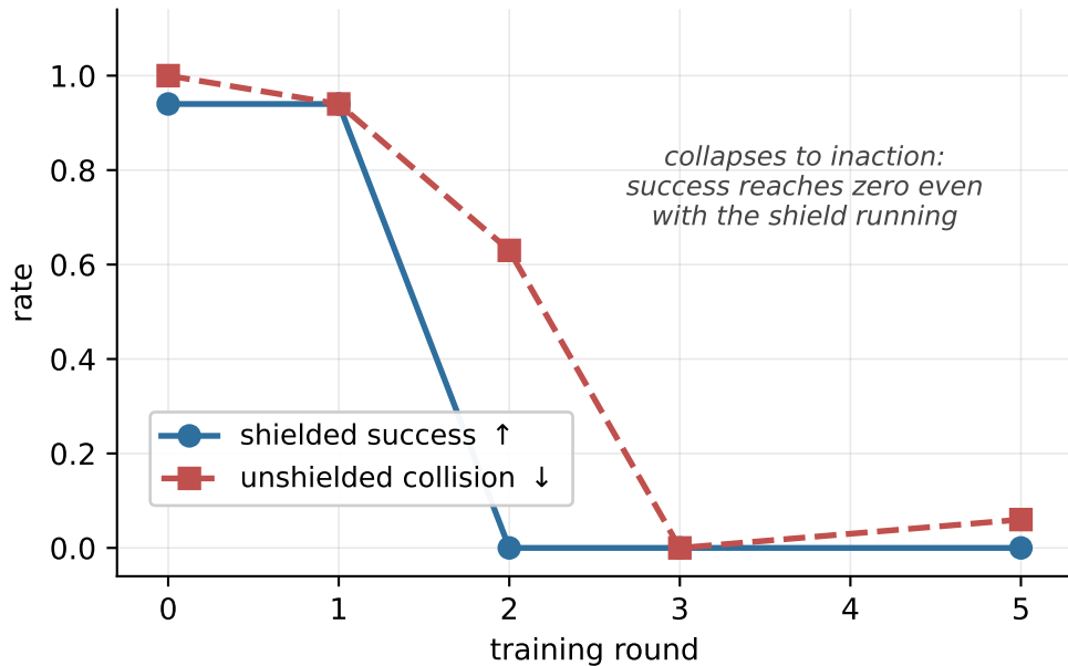
Exp 003 — collision enters the reward (lr 5 \times 10^{-5} , half rollouts unshielded)
