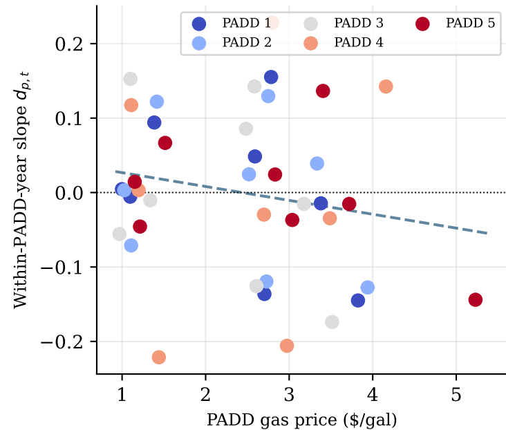
Midterms (PADD): Influence decomposition
