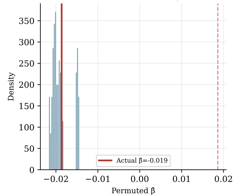
Midterms (PADD): Permutation distribution ( 5! = 120 PADD-profile perms, \rho_{perm} = 0.733 )
