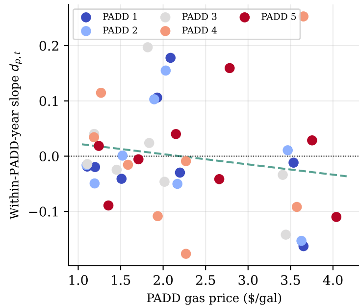
Presidential (PADD): Influence decomposition
