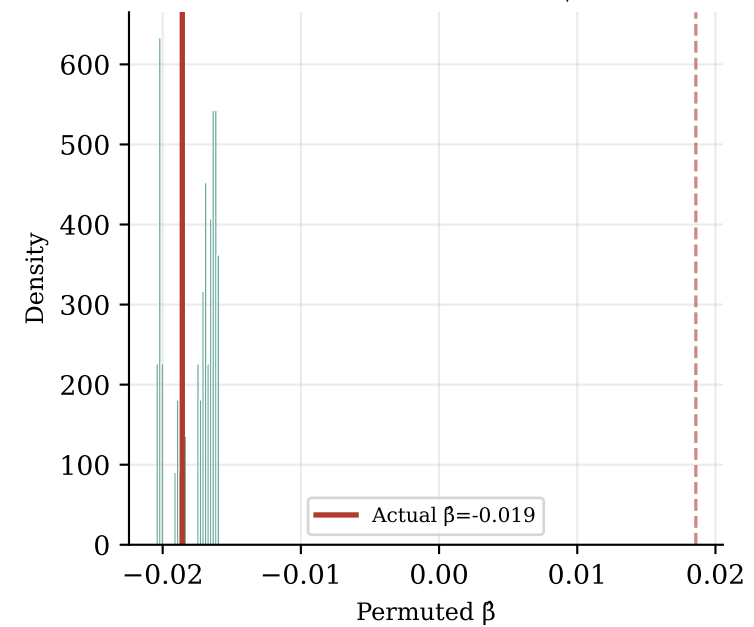
Presidential (PADD): Permutation distribution ( 5! = 120 PADD-profile perms, \rho_{perm} = 0.317 )
