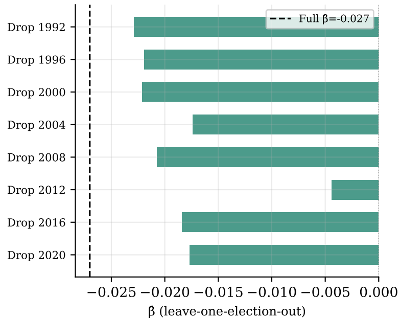
Presidential (PADD): LOEO
