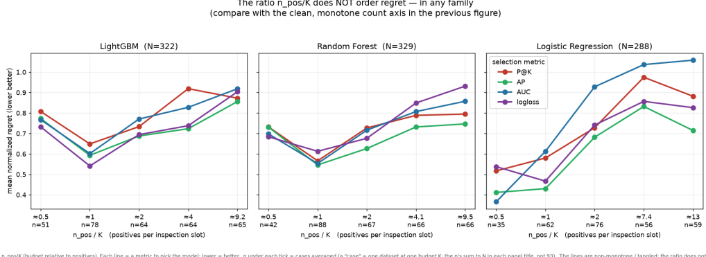
Figure 8: Regret versus the ratio n_{\text{pos}}/K , one panel per family. Unlike the count axis, the ratio does not order regret in any family — confirming that a scale-free ratio is the wrong lens.
