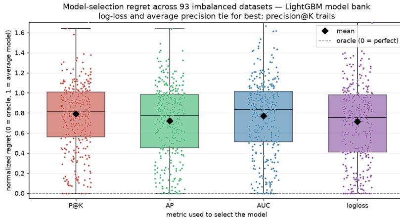
Figure 2: Distribution of normalized regret per selection metric across the 322 cases; diamonds mark means. Log-loss and average precision lead; precision@ k trails.
