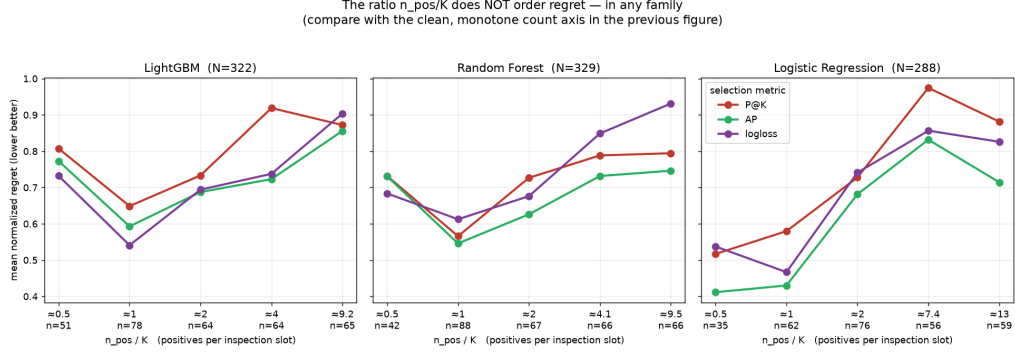
Figure 9: Regret versus the ratio n_{\text{pos}}/K , one panel per family. Unlike the count axis, the ratio does not order regret in any family — confirming that a scale-free ratio is the wrong lens.
