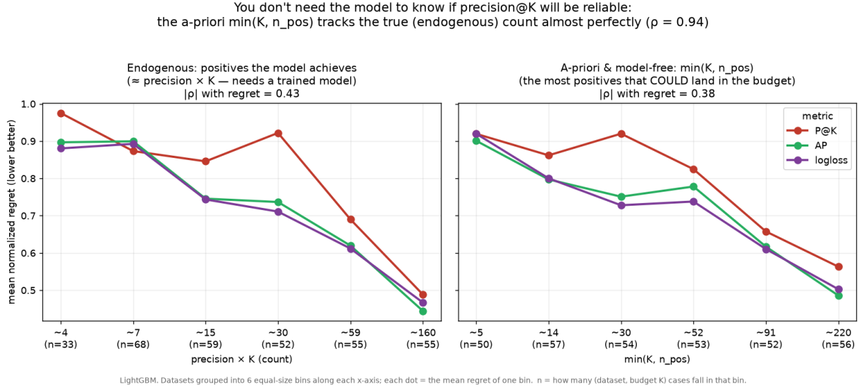
Figure 5: The endogenous count precision \times K (left) and its a-priori, model-free proxy \min(K, n_{\text{pos}}) (right) order regret almost identically ( \rho = 0.94 between them).
