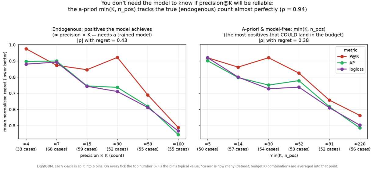
Figure 5: The endogenous count \text{precision} \times K (left) and its a-priori, model-free proxy \min(K, n_{\text{pos}}) (right) order regret almost identically ( \rho = 0.94 between them).
