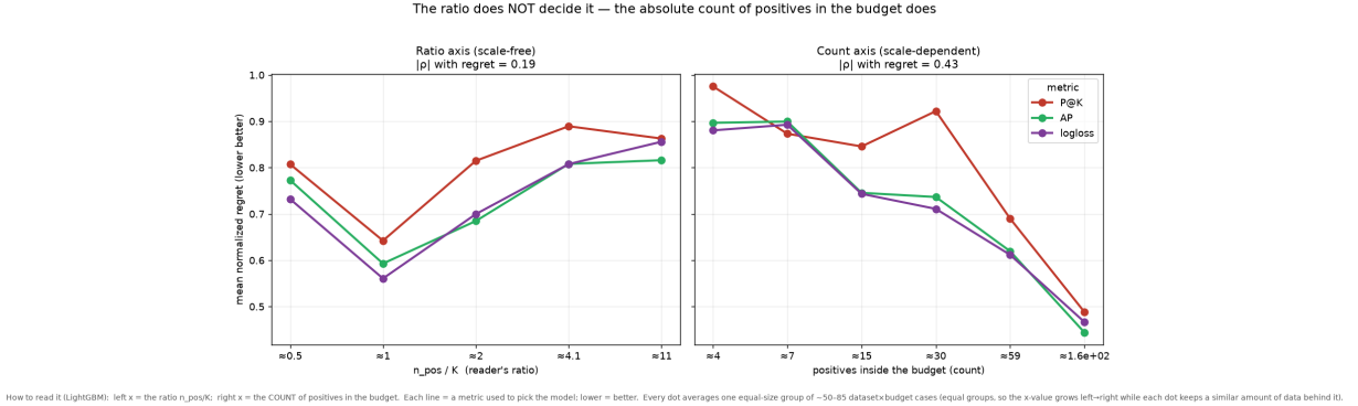
Figure 4: Left: the scale-free ratio n_{\text{pos}}/K barely orders regret. Right: the absolute count of positives inside the budget does. n = number of (dataset, budget) cases per bin.
