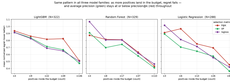
Figure 7: Mean normalized regret per selection metric, grouped by model family. Average precision (green) is lowest in all three; log-loss (purple) leads only for gradient boosting.
