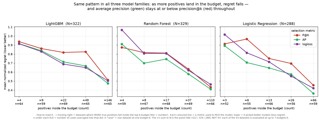
Figure 8: Regret per selection metric versus the number of true positives inside the budget, one panel per model family. In all three, regret falls as the count grows and average precision (green) stays at or below precision@k (red).
