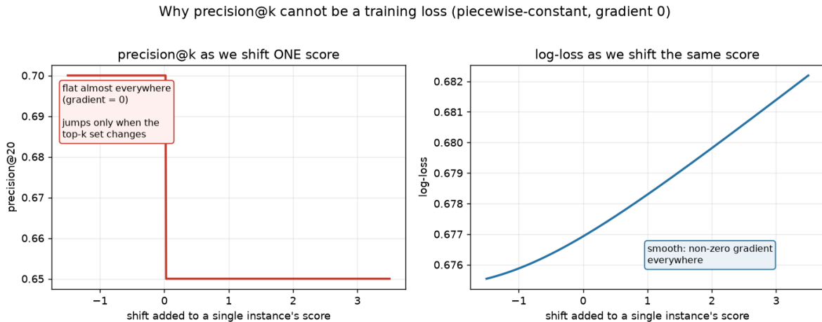
Figure 1: Sliding one item’s score: \text{precision@}k is piecewise-constant with a single cliff (gradient 0 almost everywhere), whereas log-loss is smooth with an informative gradient.
