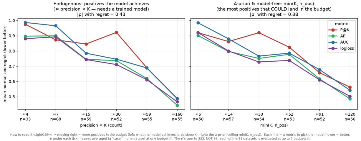
Figure 4: The endogenous count precision \times K (left) and its a-priori, model-free proxy \min(K, n_{\text{pos}}) (right) order regret almost identically ( \rho = 0.94 between them).
