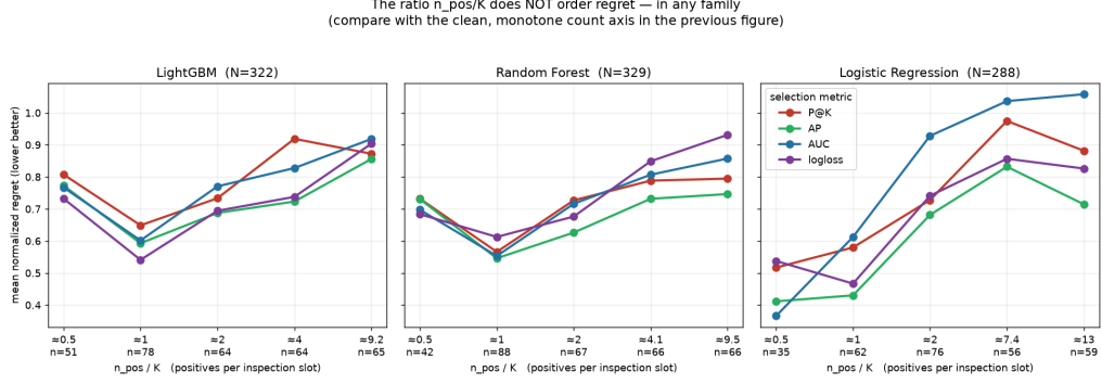
Figure 8: Regret versus the ratio n_{\text{pos}}/K , one panel per family. Unlike the count axis, the ratio does not order regret in any family — confirming that a scale-free ratio is the wrong lens.
