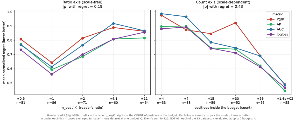
Figure 3: Left: the scale-free ratio n_{\text{pos}}/K barely orders regret. Right: the absolute count of positives inside the budget does. n = number of (dataset, budget) cases per bin.
