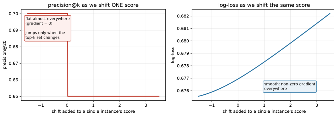
Figure 1: Sliding one item’s score: precision@ k is piecewise-constant with a single cliff (gradient 0 almost everywhere), whereas log-loss is smooth with an informative gradient.
