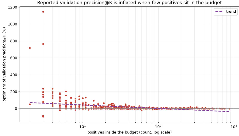
Figure 6: Optimism of validation precision@ k (over-statement of the selected model’s true precision) versus the number of positives in the budget.
