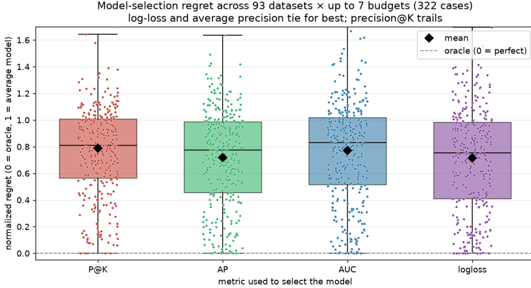
Figure 3: Distribution of normalized regret per selection metric across the 322 cases; diamonds mark means. Log-loss and average precision lead; precision@ k trails.
