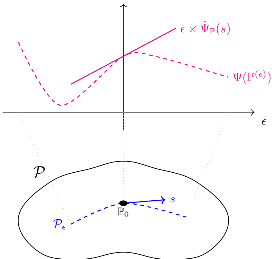
Figure 3.1: The pathwise derivative evaluated at a particular score s gives the rate of change of the estimand if we move the underlying distribution in the direction of the score.
