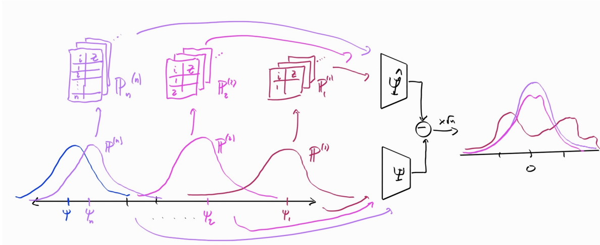
Figure 2.3: The asymptotics in the definition of regularity.
