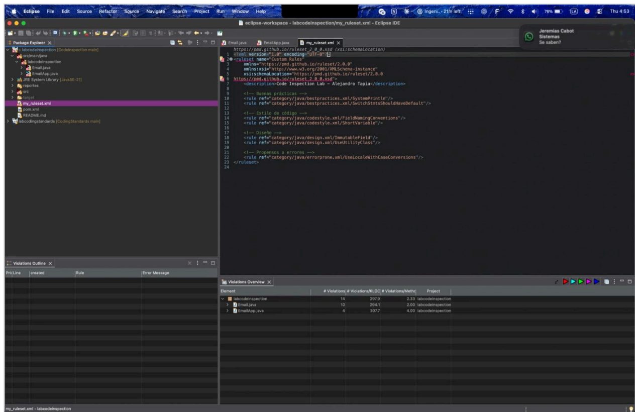
Figura 10. my_ruleset.xml.
