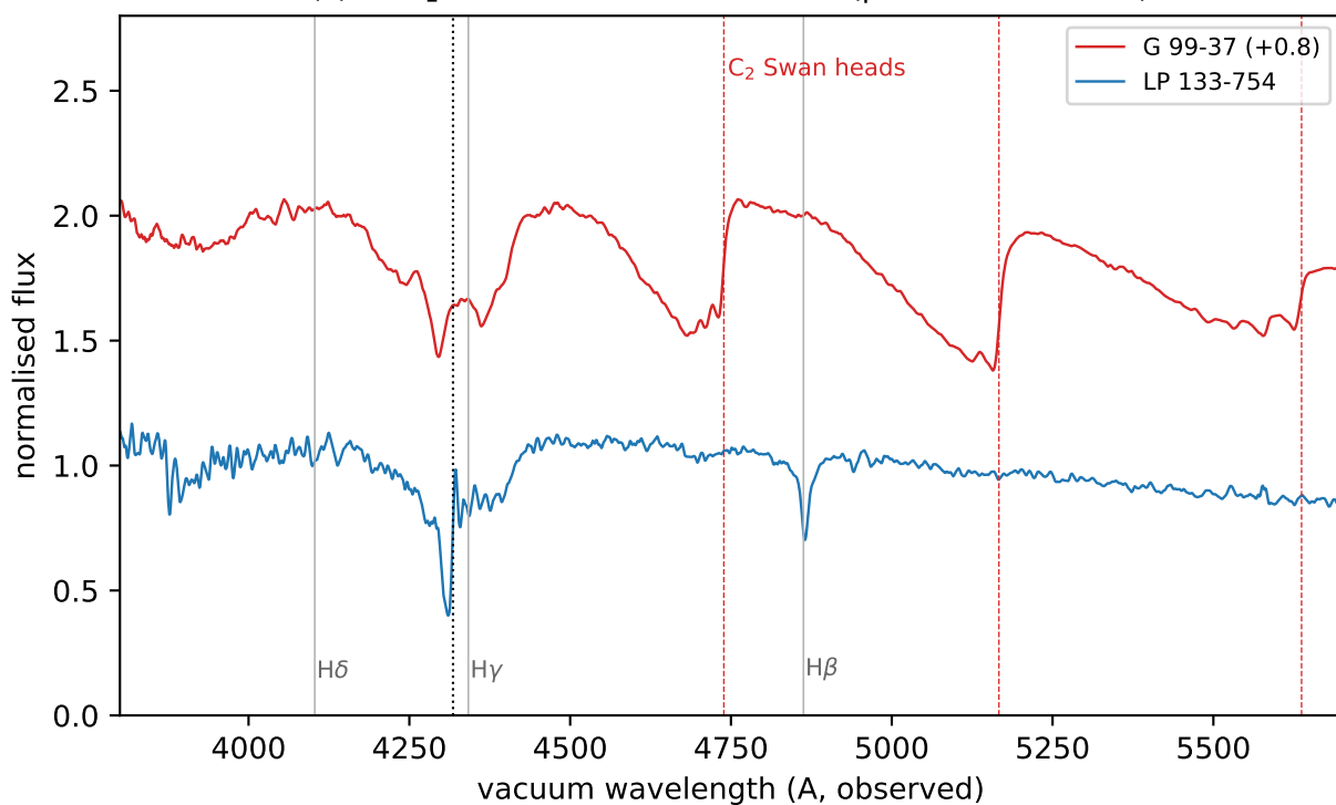
(c) no C 2 Swan bands in LP 133-754 (present in G 99-37)
