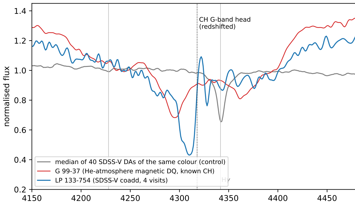
(a) CH G band: LP 133-754 vs control DAs and G 99-37
