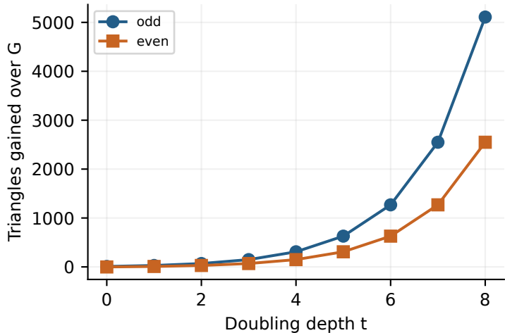
Exact improvement over the baseline
