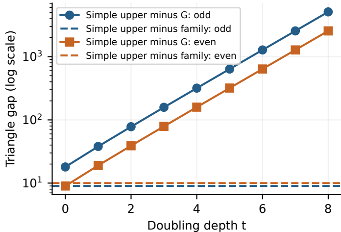
Constant family gaps
