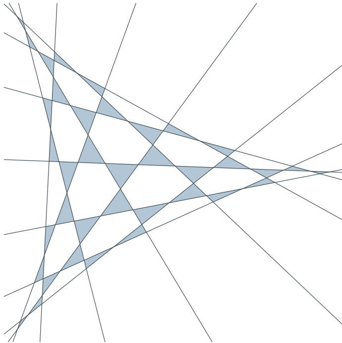
\alpha = 1/6 : 37 cells
