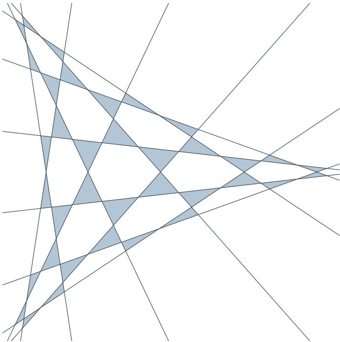
\alpha = 1/2 : 36 cells
