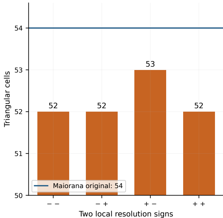
A 14-line smoothing counterexample
