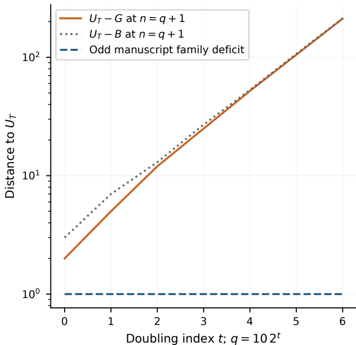
Sparse odd family versus all-order formulas
