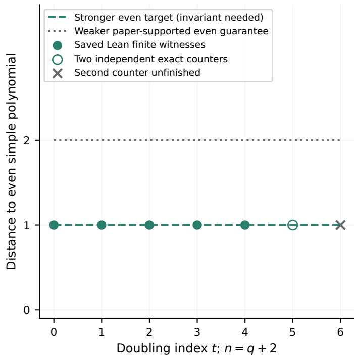
Even companion: verification is not uniform
