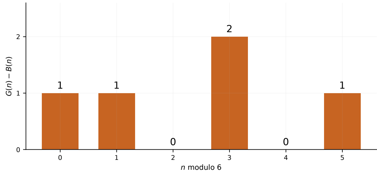
Exact gain by residue class, for n \geq 4
