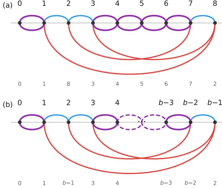
Figure 2: The odd gadget H_{T'_b} : (a) the instance T'_9 = (0, 1, 8, 3, 4, 5, 6, 7, 2) ; (b) general odd b , the middle of the highway elided. Conventions as in Figure 1. Note the contrasts with H_{T_b} : vertex 0 is a leaf (its doubled pair \{0, 1\} is its only edge pair), the terminal v_1 sits at vertex 2, and the doubled run D = \{3, \dots, b-2\} is one vertex shorter than the segment of H_{T_b} – the relabeling that reverses the good parity from even to odd b .
