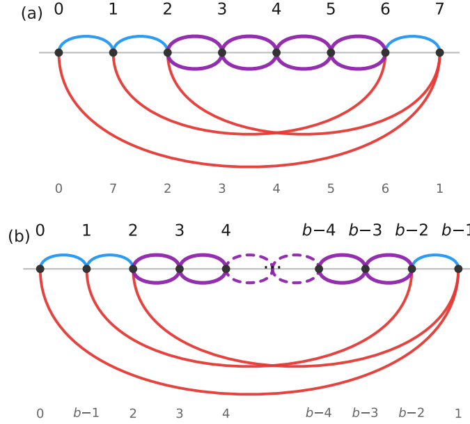
Figure 1: The gadget H_{T_b} : (a) the instance T_8 = (0, 7, 2, 3, 4, 5, 6, 1) ; (b) general even b , the middle of the segment elided. Vertices are positions on a line, with the value T_b(i) in small gray below; blue arcs above the line are P-edges, red arcs below are V-edges, and a purple pair of mirrored arcs is a doubled pair. The doubled run on the segment S = \{2, \dots, b-2\} is flanked by the three P-only edges \{0, 1\}, \{1, 2\}, \{b-2, b-1\} and the three V-only edges \{0, b-1\}, \{2, b-1\}, \{1, b-2\} ; the terminals are 0 ( = p_0 = v_0 ), 1 ( = v_1 ), and b-1 ( = p_1 ).
