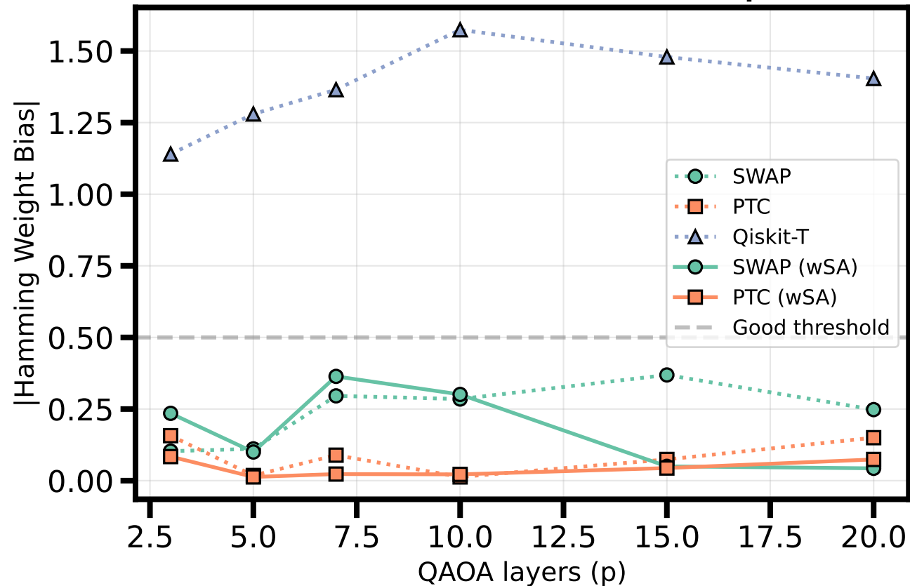
Bit Distribution Bias vs Circuit Depth
