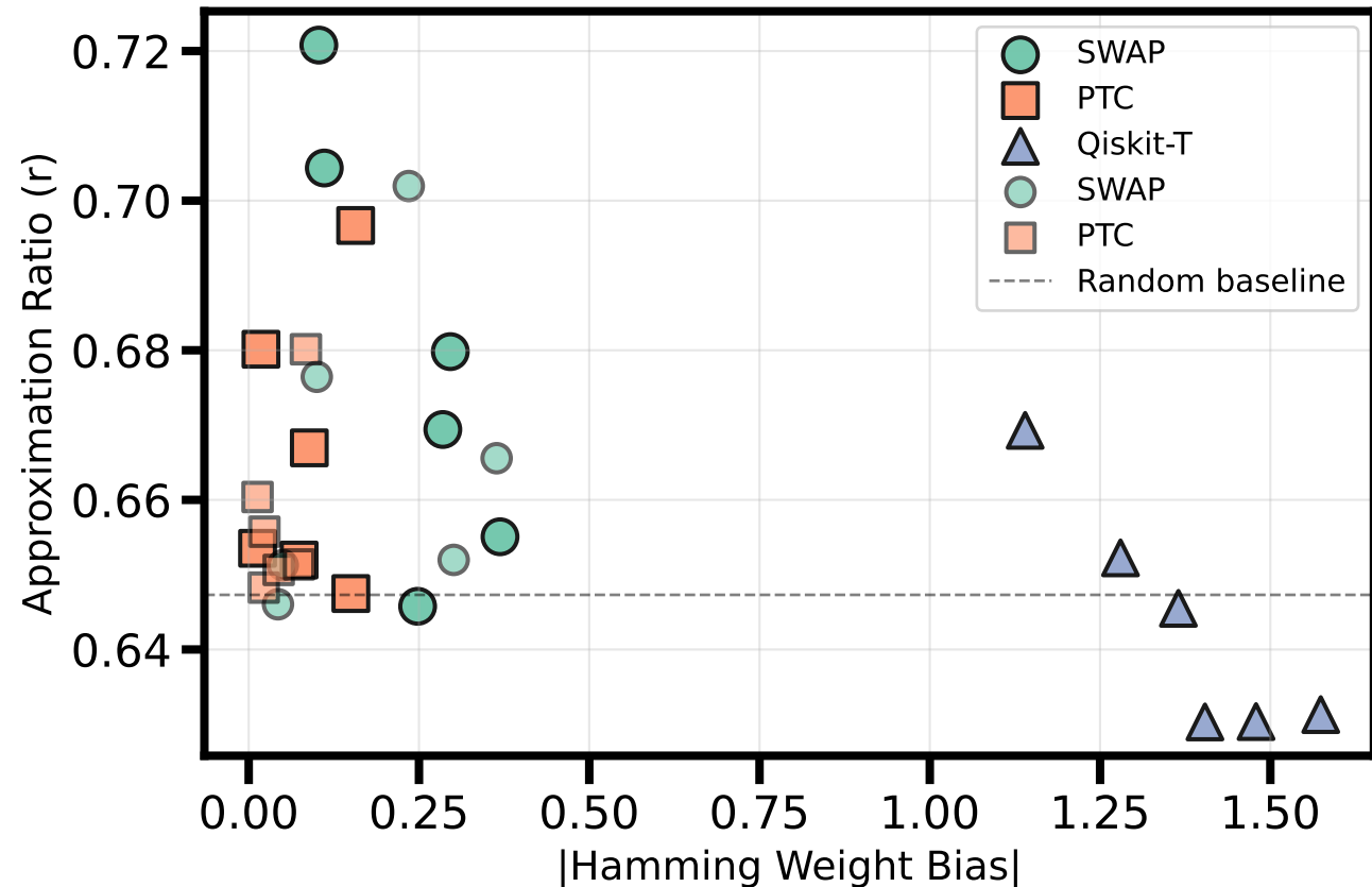
Performance vs Bit Distribution Bias
